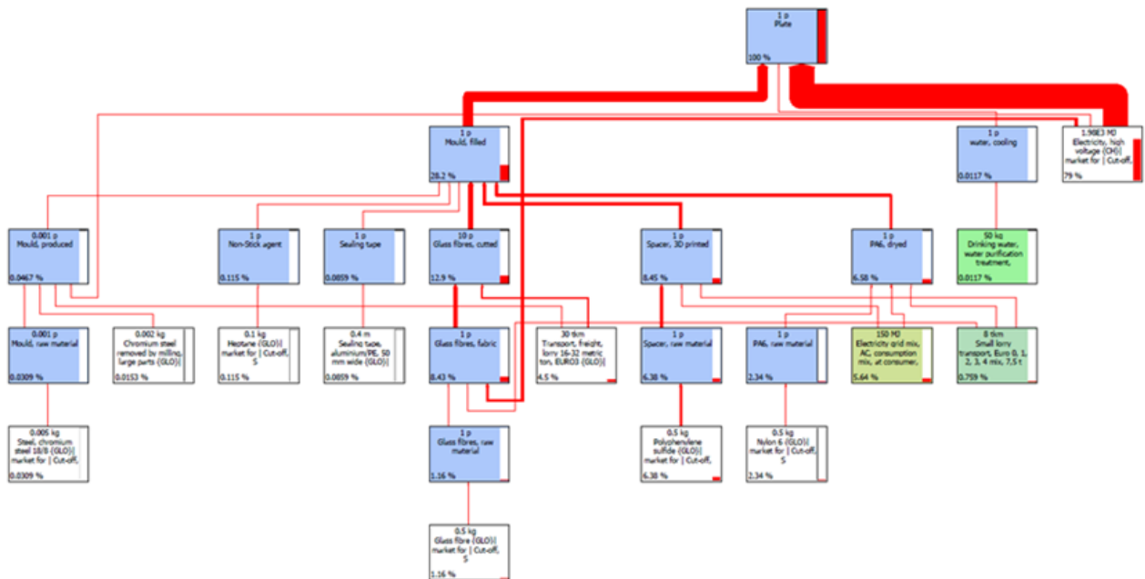
Exemplary energy flow for the production of a plate produced by melt-resin transfer molding (in plane) at EPFL taken from SimaPro.
