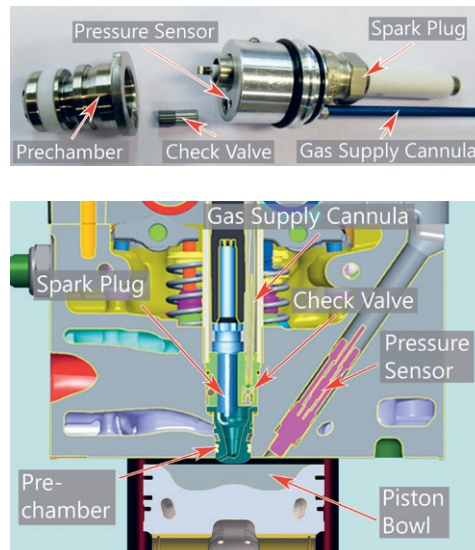
Concept of the novel turbocharged pre-chamber gas engine.
