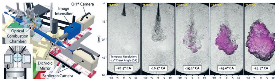
Left: Test setup with cameras.
