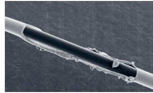
Open coating bicomponent fiber.
