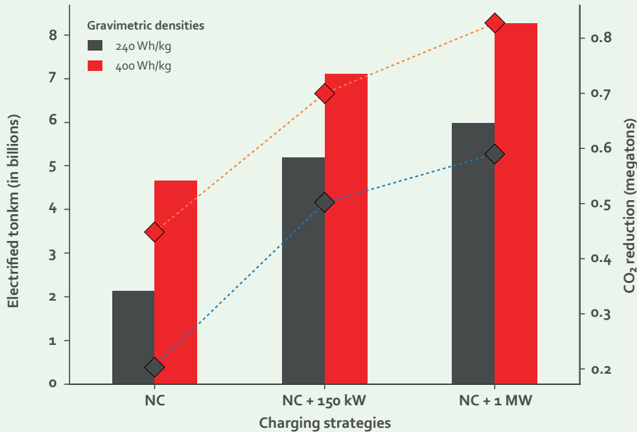
Number of ton kilometers (tonkm) that could be covered by battery electric trucks given different energy densities of batteries and charging strategies, along with CO 2 emissions avoided.
