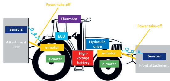
Rigitrac's electric tractor was awarded the Swiss Innovation Award 2018 by the Swiss Agricultural Engineering Association.
