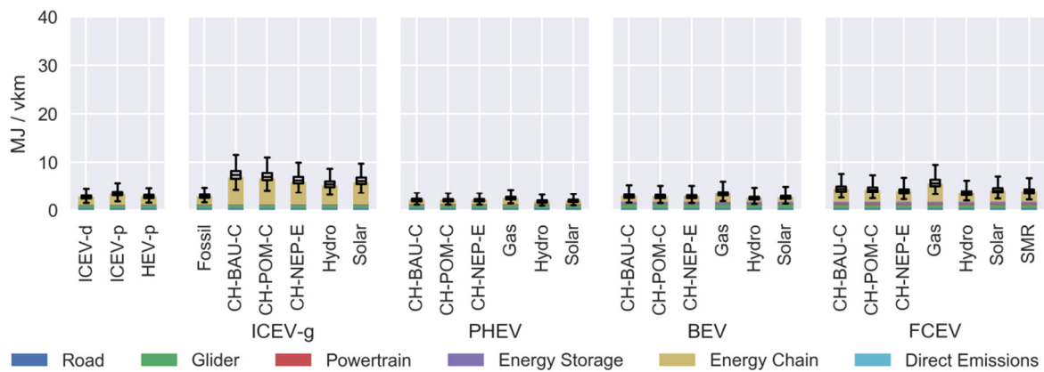
Figure 14 Vehicle cumulative energy demand results for future vehicles. Bar chart shows most likely result; whisker plot shows variability due to different vehicle design and uncertainty of future performance.
